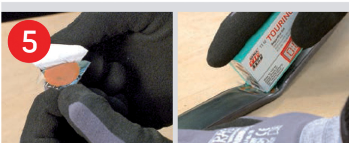
5 Remove the aluminum protection foil from the patch, place it on the repair area and immediately press firmly
