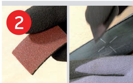
2 Buff the repair area slightly larger than the patch size
